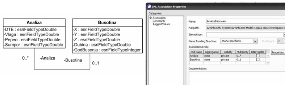
Figure 3 - Binary association between Busotina and Analiza classes
