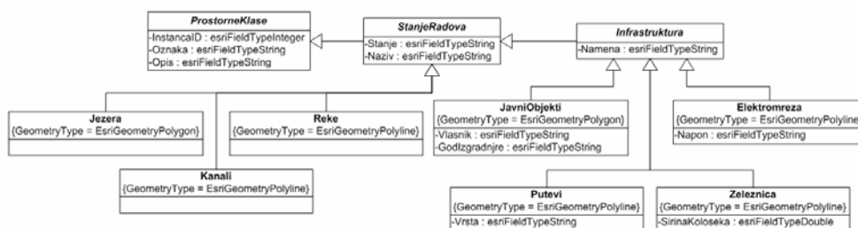
Figure 4 - Class diagram Objekti
