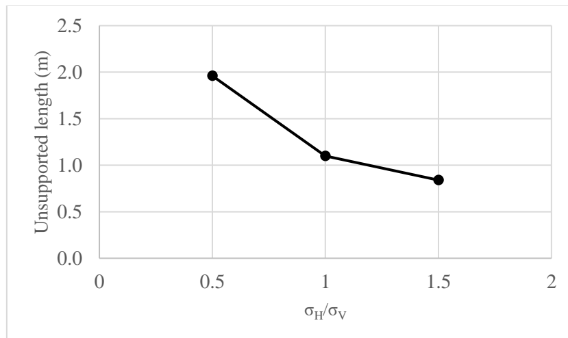
Figure 8 Unsupported length vs stress ratio
