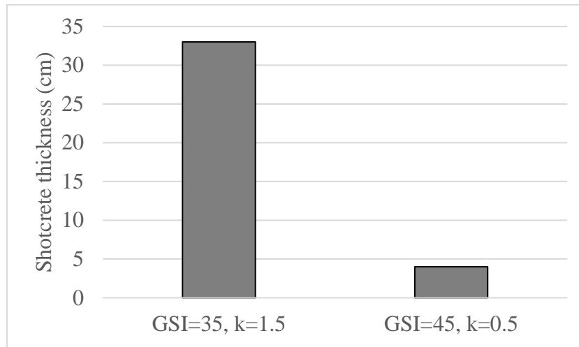
Figure 11 Shotcrete thickness for best- and worst-case
