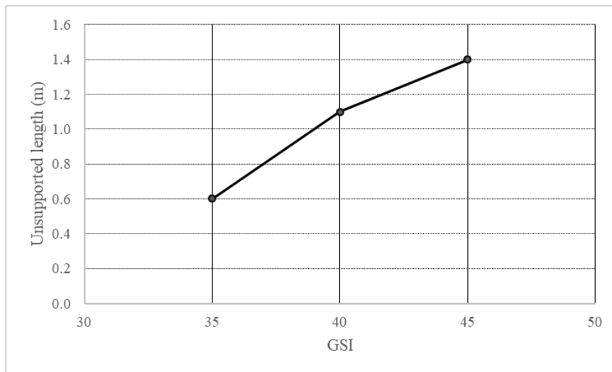
Figure 6 Unsupported length vs GSI change
