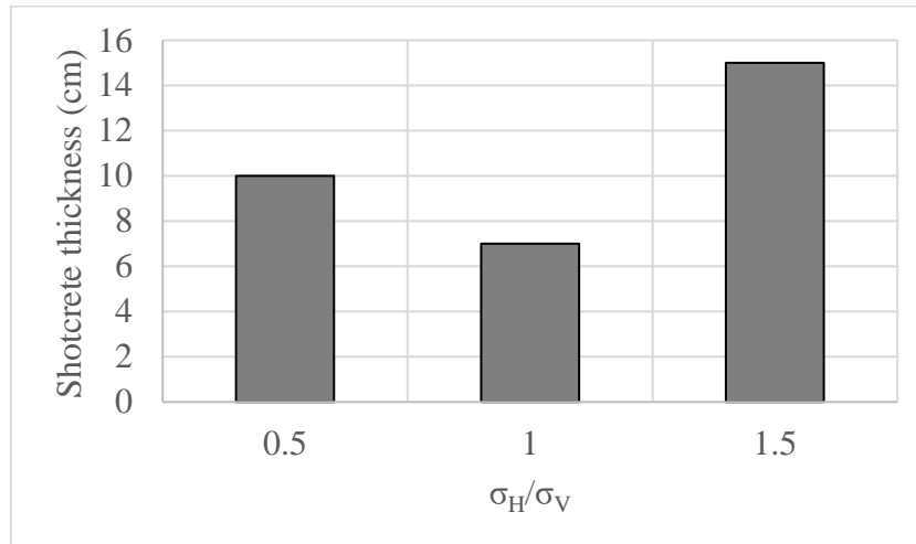
Figure 9 Shotcrete thickness vs stress ratio
