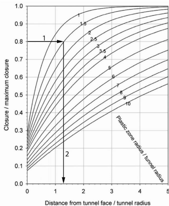
Figure 5 Diagram by Vlachopoulos and Diederichs (2009)
