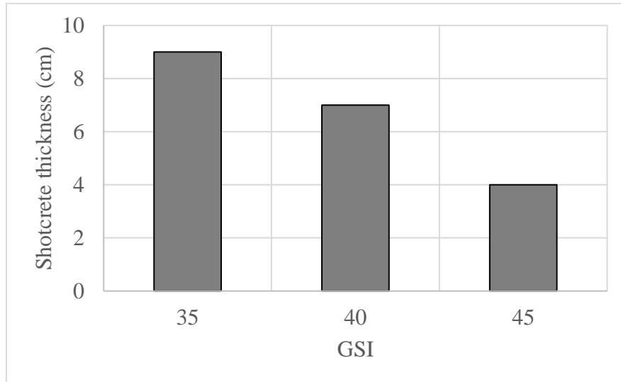
Figure 7 Shotcrete thickness vs GSI change
