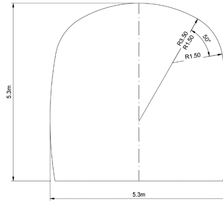
Figure 1 Decline cross section
