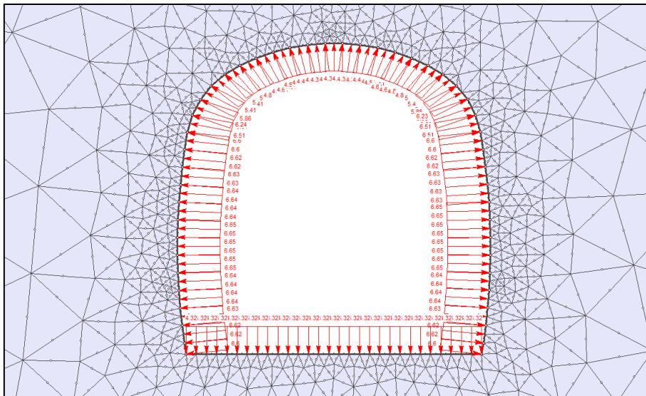
Figure 2 Distributed load at excavation boundary
