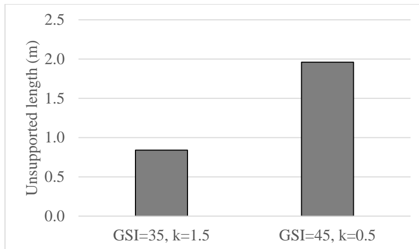
Figure 10 Unsupported length vs stress ratio
